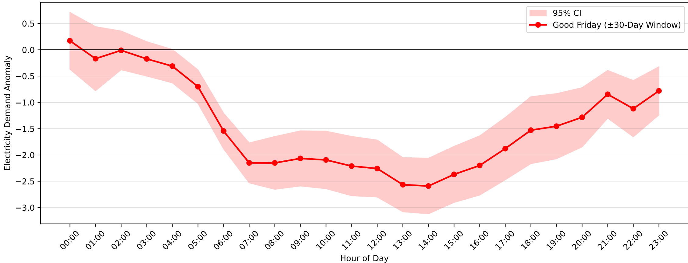
Gateshead Demand Anomaly: Good Friday (2004–2017, \pm 30 -Day Window)
